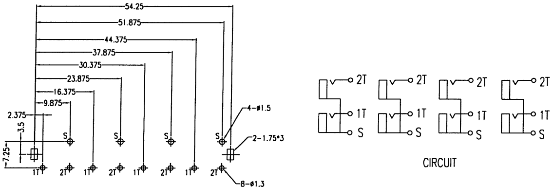
T:1.6 Dimensions of PC board holes Tolerance : ±0.1(Printed-side view)
