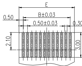
FPC LAYOUT (THICKNESS:0.3±0.03)
