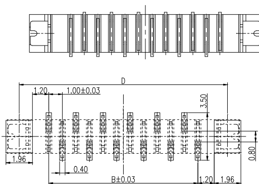
PCB LAYOUT (REF)
